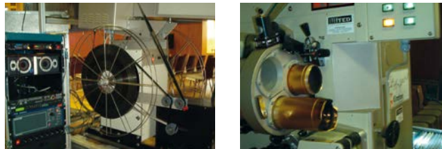
Motion picture projection using the analogue 35 mm technology
